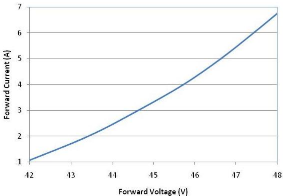
(i) Typical Forward Current ( I_F ) vs. Forward Voltage ( V_F ) of Red Section
